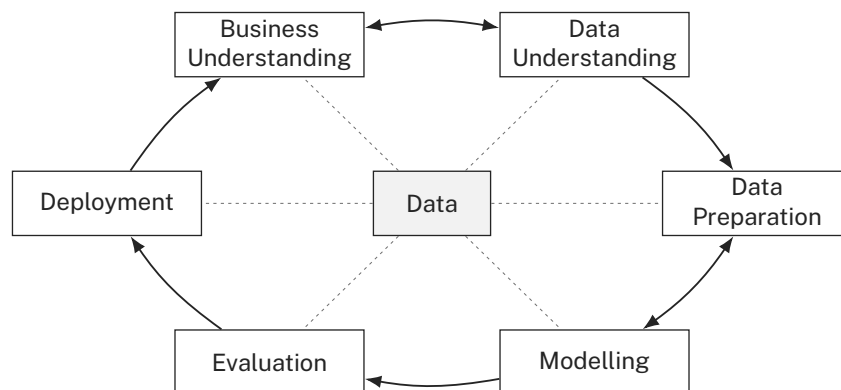
Figure 2. The six CRISP-DM stages. The cycle runs clockwise from business understanding, the two double-headed arrows mark the pairs that are worked back and forth, and every stage reads from and writes to the same data.
